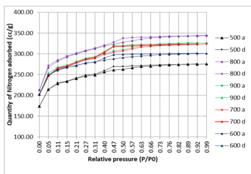
Figure S3. Nitrogen adsorption and desorption isotherms at 77K for the PVDF-derived porous carbon adsorbents at different temperatures
